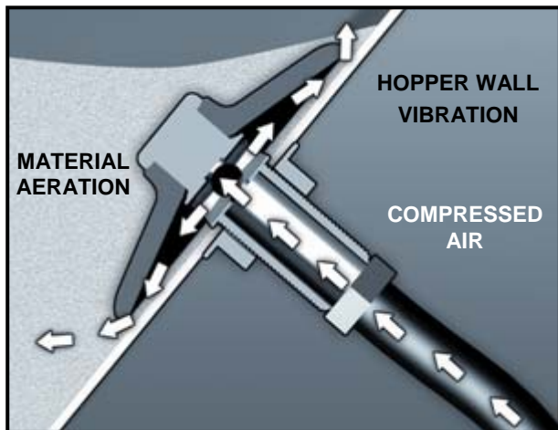
Hopper cutaway showing fluidizer action
