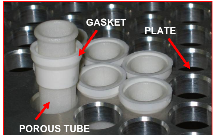
CLOSE UP OF FILTER TUBES MOUNTED IN A MACHINED ALUMINUM PLATE
