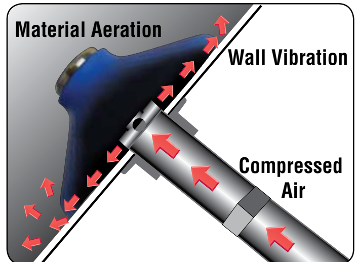
Hopper cutaway shows Fluidizer in use.
